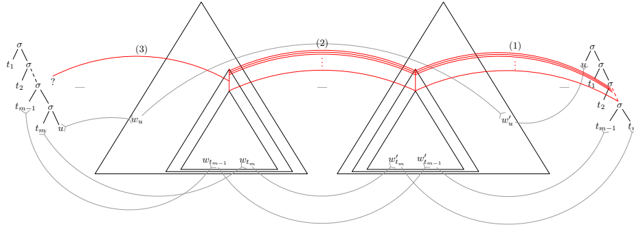
Fig. 4. Illustration of the dependencies discussed in the proof of Theorem 6. Inverted arrow heads indicate that the link points to a position below the one indicated by the spline. The links relating the roots of the trees are omitted.
