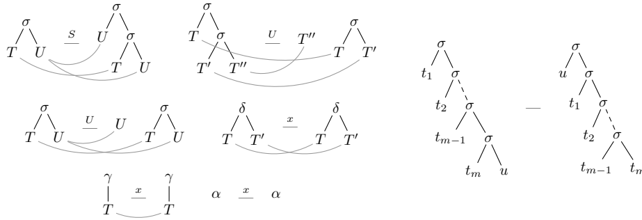
Fig. 3. Productions of the counterexample MBOT Tpc with x \in \{T, T', T''\} and relation (topicalization) computed by it for all m \in \mathbb{N} and arbitrary trees u, t_1, \dots, t_m , which can contain binary \delta -symbols, unary \gamma -symbols, and nullary \alpha -symbols.
