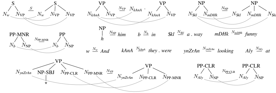
Fig. 1. Example productions.
