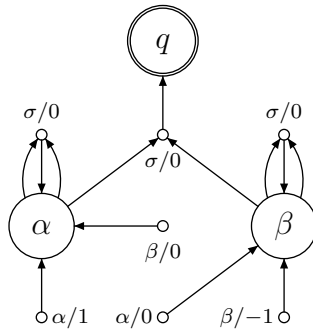
Figure 1: Bu-w-fta M which recognizes a tree series/fuzzy set with a non-recognizable cut set.
