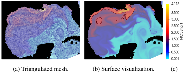
Figure 4: Figure 4a shows the triangulated mesh obtained from the particle locations at t = 6.25 days, and Figure 4b shows the surface rendering of the Delauney mesh. An isocontour of NO_{3,t_0} = 1.8 \text{ mmol m}^{-3} is presented on top showing regions with high NO_{3,t_0} values.
