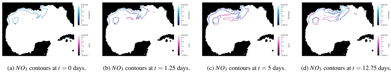
Figure 11: Visualization of superimposed NO_{3,t_0} contours extracted from Lagrangian advection (blue contours), and Eulerian scalar NO_3 data (red contours). Figure 11a shows the contours at initial time t = 0 days. At this time we start the advection and consequently both the contours overlap each other. Figure 11b shows the result at t = 1.25 days where we observe regions that have both red and blue contours and are concluded to be the result of surface advection. Figure 11c depicts contours at t = 5 days. At this time, we see red contours which do not overlap with any blue contours and hence are suspected as the result of vertical mixing and upwelling. Figure 11d shows results from a later time, where upwelling is observed in a different region of the ocean.
