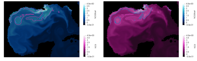
Figure 6: Comparative visualization of NO_3 contours with NO_3 distributions from different sources are shown in the background as a context.
