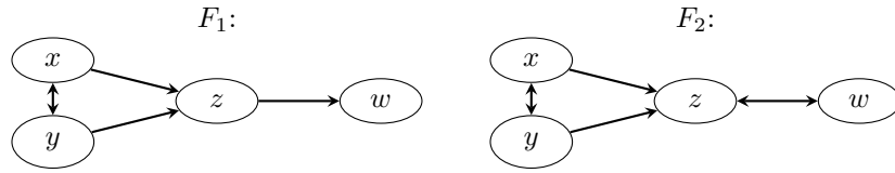
Figure 3: Two argumentation frameworks F_1, F_2 . In both, the grounded extension is empty, and argument w is contained in every preferred extension. The ideal semantics can distinguish between the two, since in F_1 argument w cannot defend itself (ideal extension \emptyset ) while in F_2 it can (ideal extension \{w\} ).
