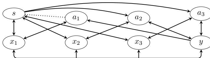
Figure 2: Orientation of attacks due to previously non-explicit conflicts matters: First observe that st(F) = \{\{a_1, a_2, x_3\}, \{a_1, a_3, x_2\}, \{a_2, a_3, x_1\}, \{s, y\}\} . Next, Pairs_{st(F)} yields one pair of arguments a_1 and s whose conflict is not explicit by F , that is, (a_1, s) \notin Pairs_{st(F)} , but (a_1, s), (s, a_1) \notin R_F . Now adding the attack (a_1, s) to F would create the additional stable extension \{a_1, a_2, a_3\} \notin st(F) . On the other hand, by adding the attack (s, a_1) , we get the conflict-explicit AF F' with st(F) = st(F') .
