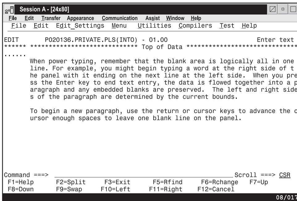
Figure 100. Sample Text During Text Entry Mode.
