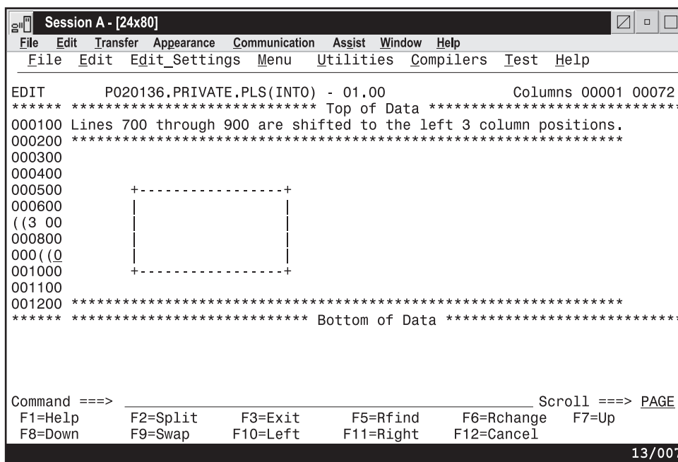
Figure 57. Before the ( (Column Shift Left) Line Command
