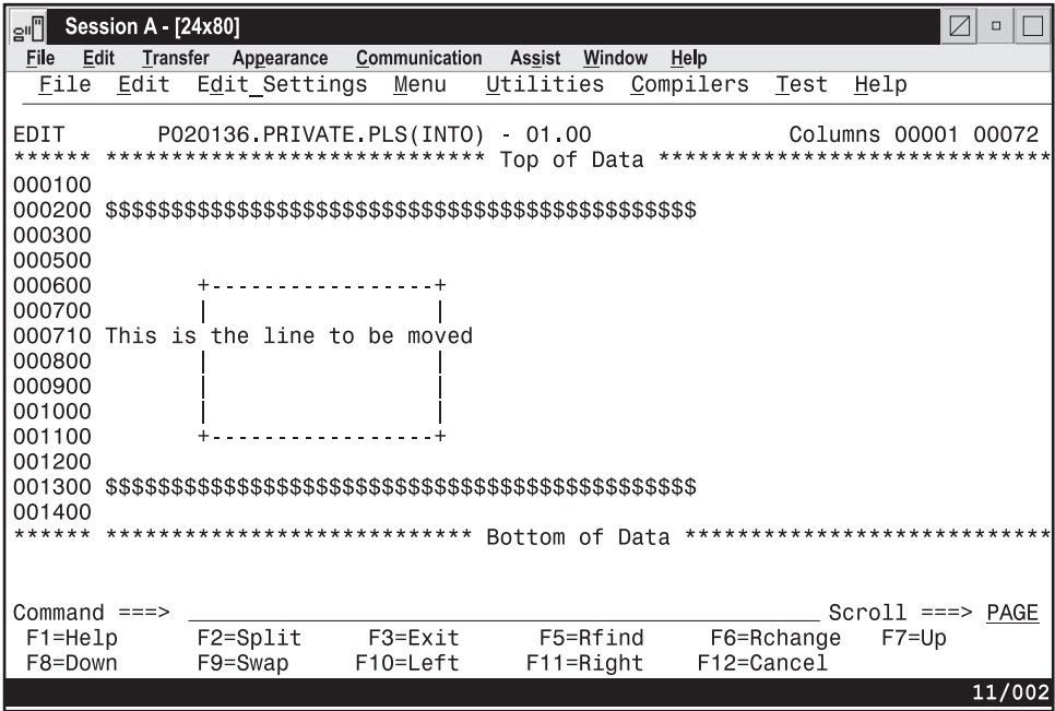
Figure 86. After the M (MOVE) Line Command
