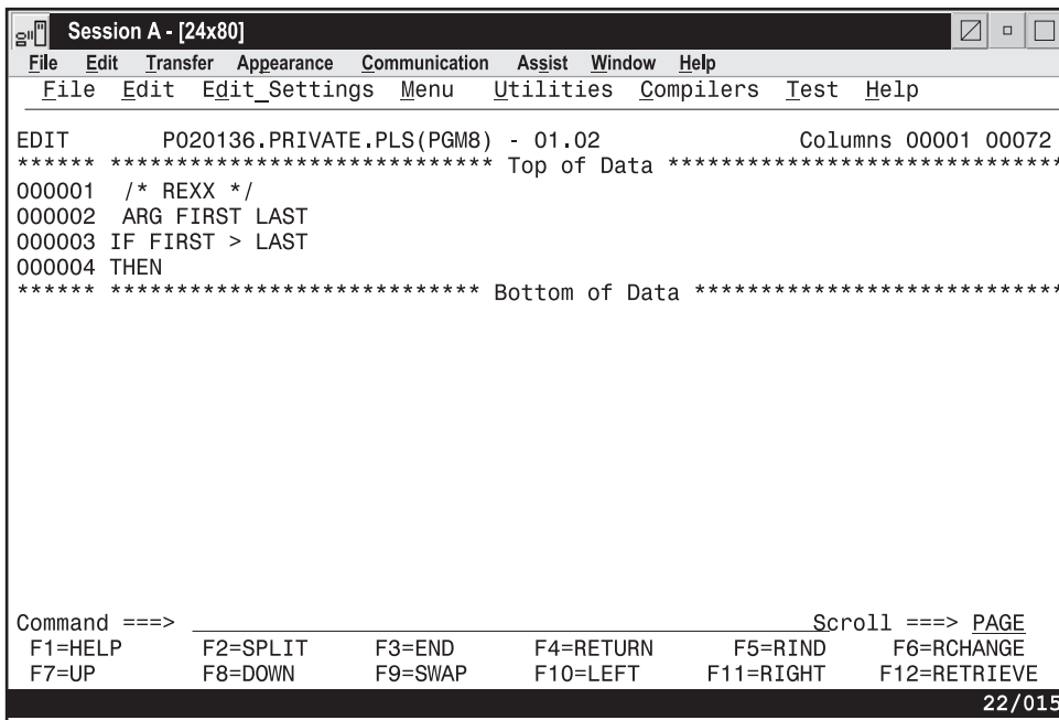
Figure 154. Member After Lines Are Unnumbered
