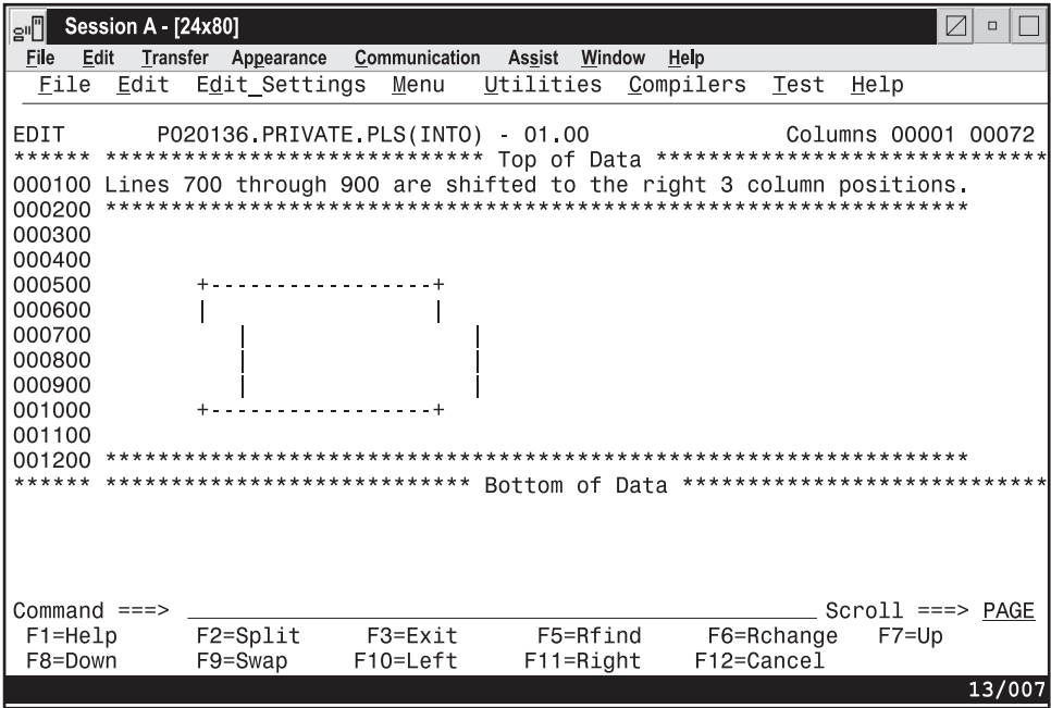
Figure 60. After the ) (Column Shift Right) Line Command
