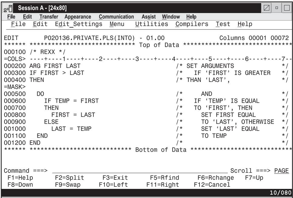
Figure 88. After the MASK Line Command
