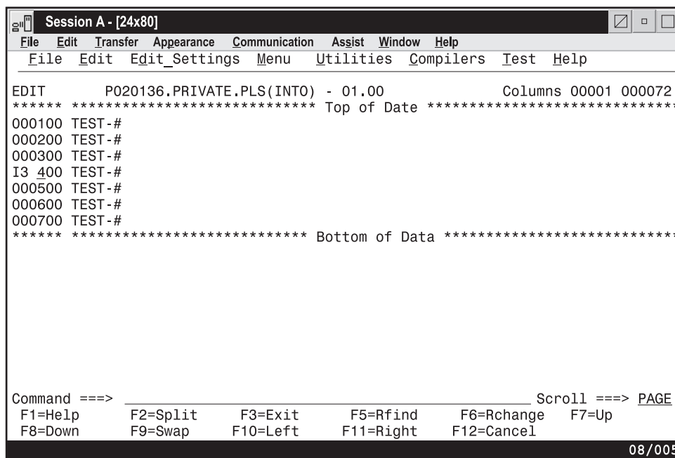
Figure 79. Before the I (Insert) Line Command
