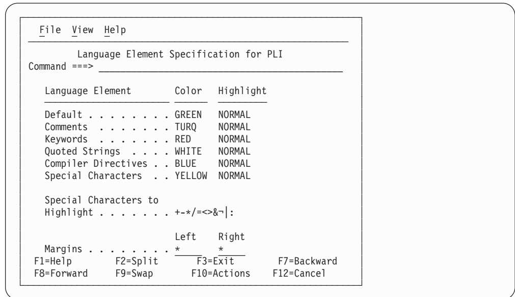
Figure 10. HILITE Language Element Specification Screen (ISREPC1)
