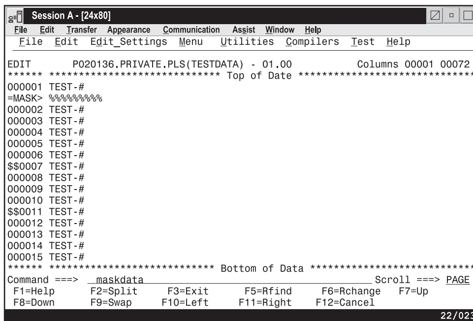
Figure 55. ISRMASK Macro - Before Running
