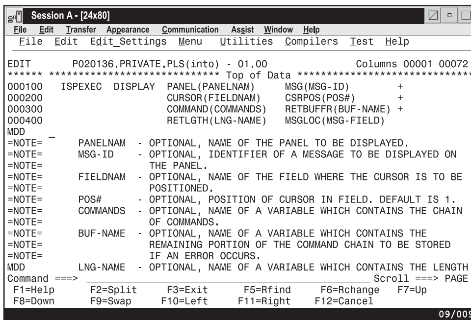
Figure 89. Before the MD (Make Dataline) Line Command
