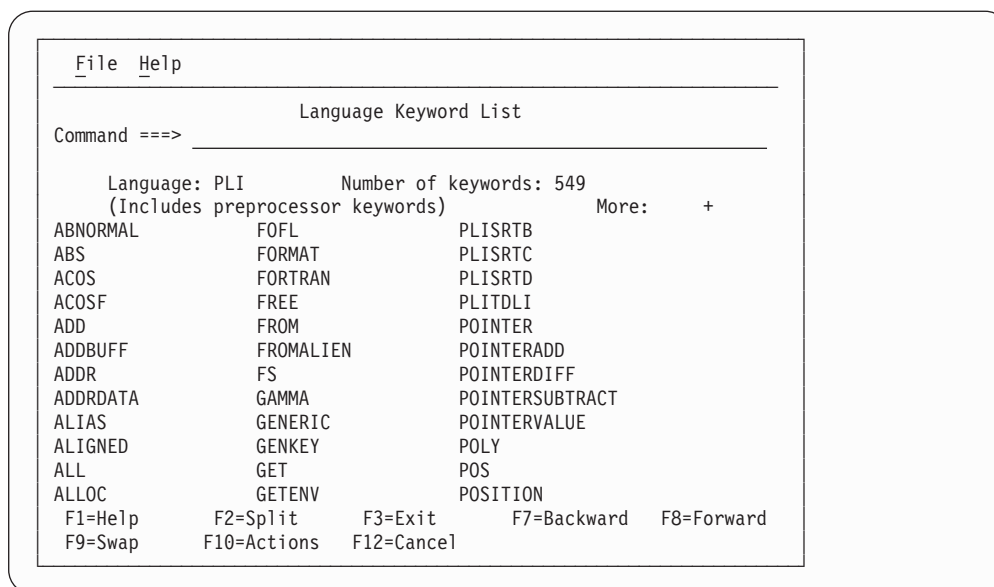
Figure 11. HILITE Language Keyword List (ISREPK)
