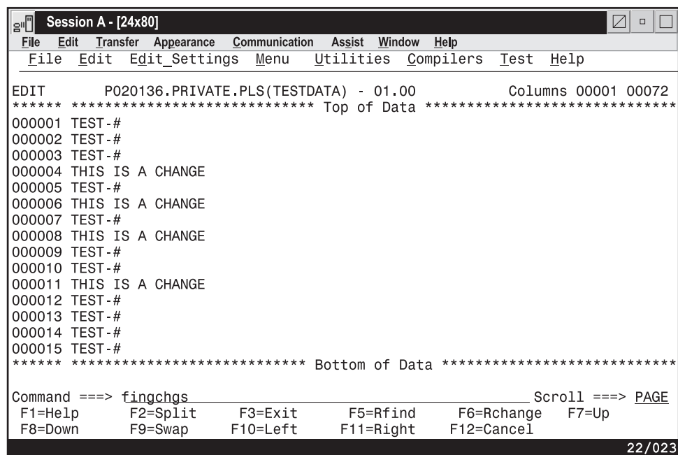
Figure 52. ISRCHGS Macro - Before Running
