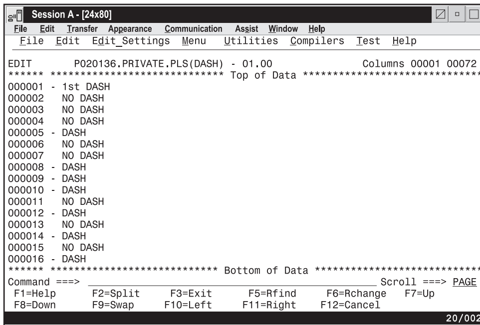
Figure 28. ISRDASH Macro - Before Running
