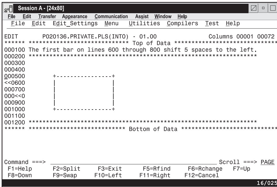
Figure 61. Before the < (Data Shift Left) Line Command
