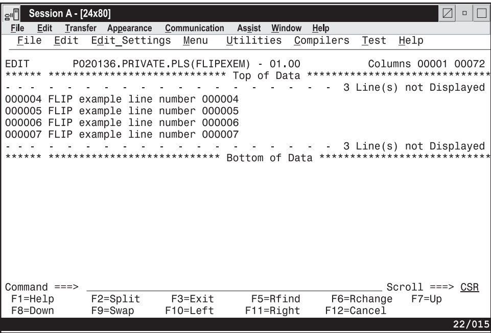
Figure 127. Example of Data Set using FLIP on Excluded Lines
