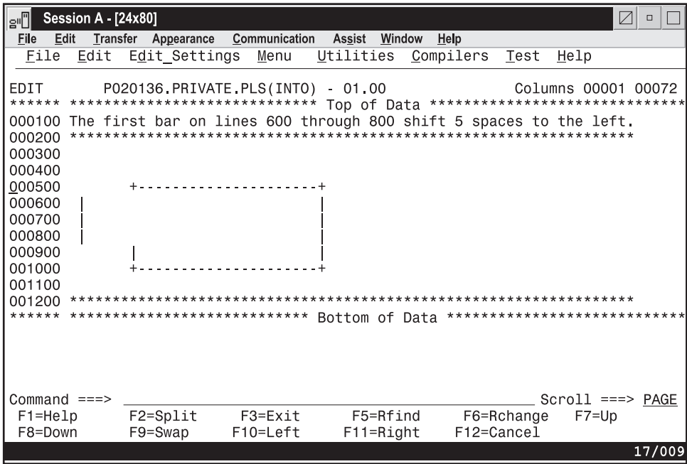
Figure 62. After the < (Data Shift Left) Line Command
