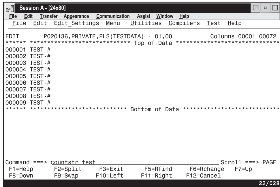
Figure 34. ISRCOUNT Macro - Before Running
