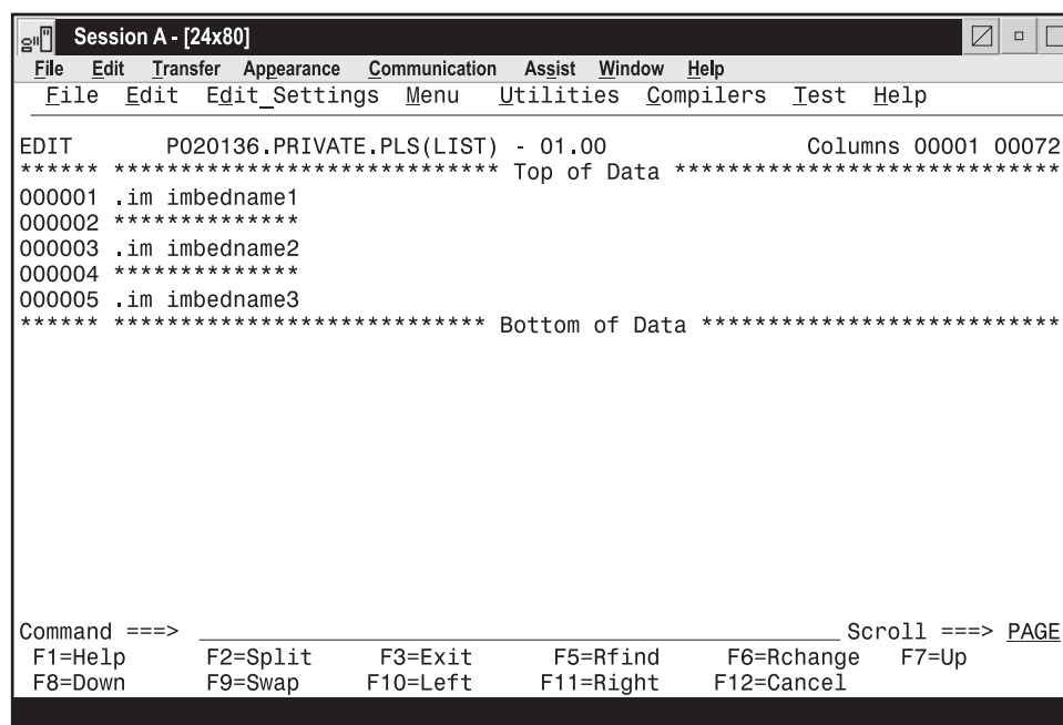
Figure 48. LIST with Imbed Statements
