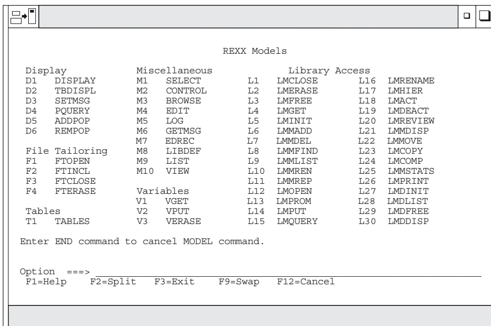
Figure 136. REXX Models Panel (ISREMRXC)
