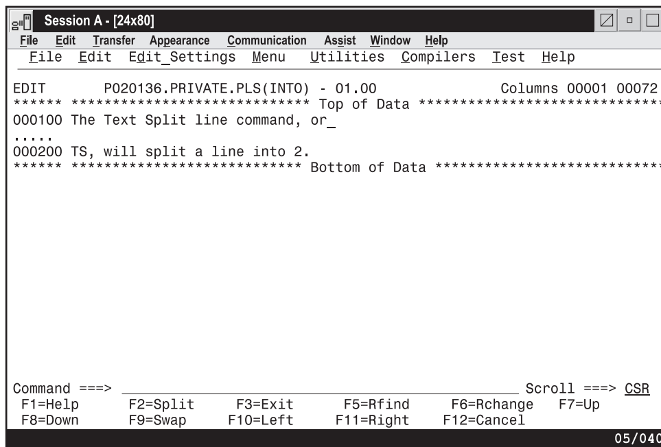
Figure 105. After TS (Text Split) Line Command
