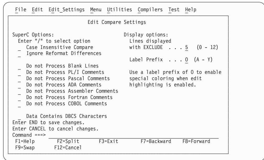
Figure 111. Edit Compare Settings Panel
