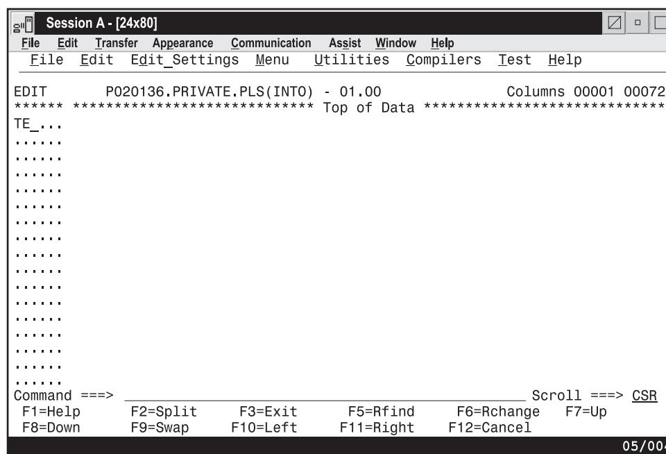
Figure 98. Before the TE (Text Entry) Line Command
