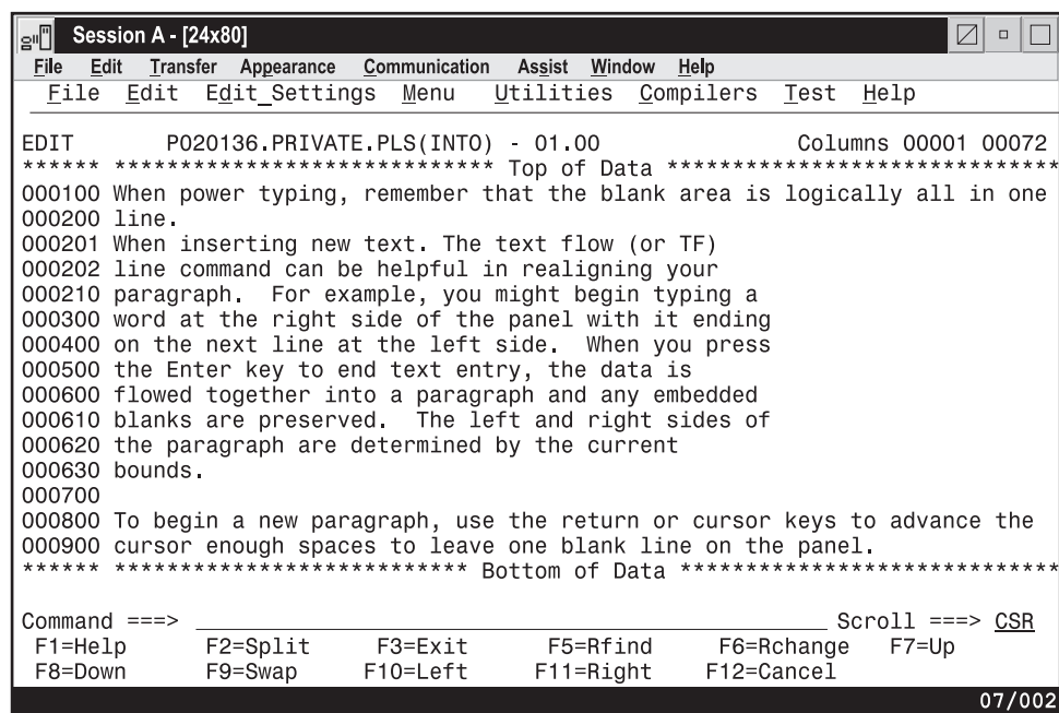
Figure 103. After the TF (Text Flow) Line Command
