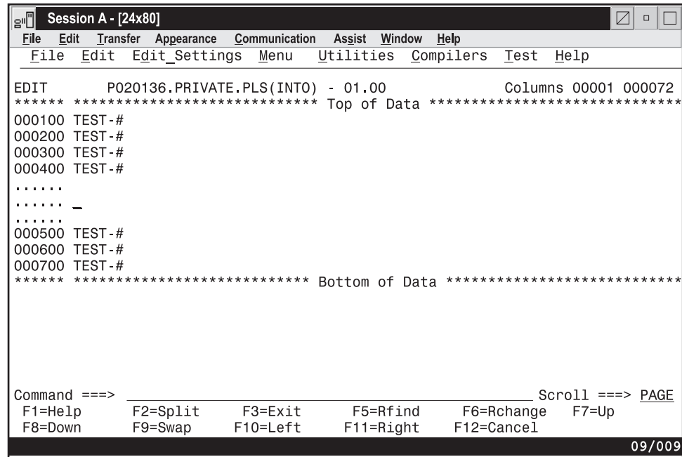
Figure 80. After the I (Insert) Line Command
