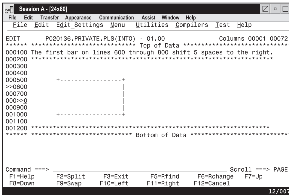
Figure 63. Before the > (Data Shift Right) Line Command
