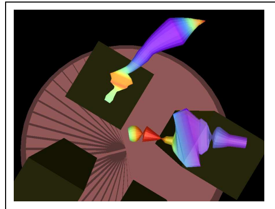
Figure 10. Minor hyperstreamlines for four-pile group data set. Varying diameter indicates problems with other two eigenvector fields.
