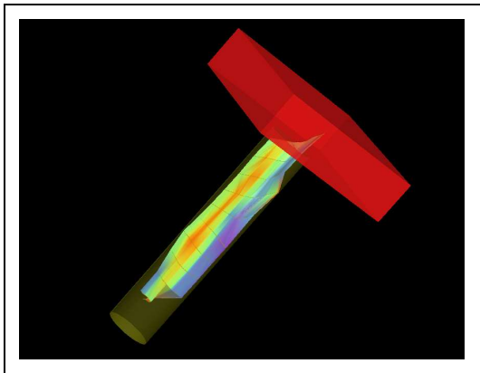
Figure 13. Minor hyperstreams-surfaces limited to concrete pile. Behavior of a family of minor tensor lines starting at center line of pile becomes evident.
