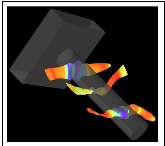
Figure 9. Major hyperstreamlines for one-pile data set.
