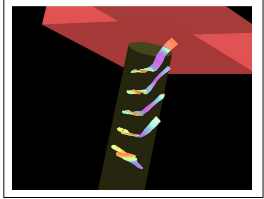
Figure 8. Minor hyperstreamlines for one-pile data set. Varying diameter illustrates rapid changes in other two eigenvalues.
