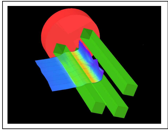
Figure 14. Minor hyperstreams-surfaces visualizing behavior of a family of minor tensor lines for four-pile-group data set. (We have removed one of the piles to simplify the view.)
