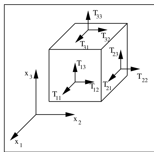
Figure 2. Definition of stress tensor.
