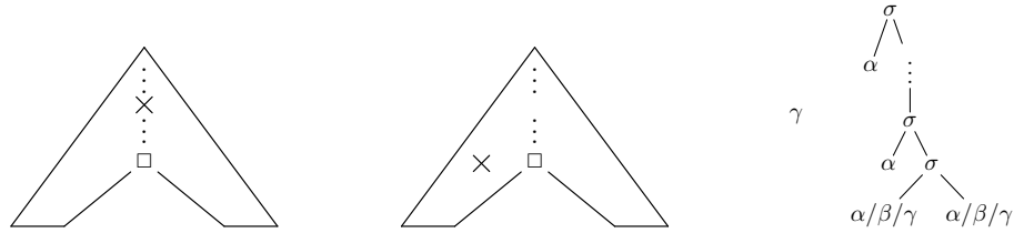
Fig. 1. Illustration of the difference locations in a context: along the path to the root (left) and off this path (middle), and illustration of the tree language L(M_{\text{ex}}) of Ex. 2.
